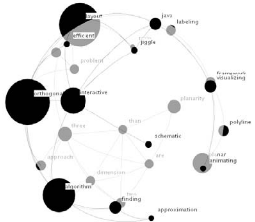
Figure 10: Layouts of the title-word graph with different centers of attention in spherical space.
