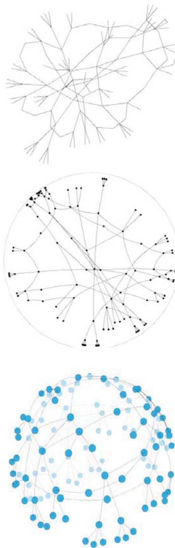
Figure 1: Drawings of the same simple, undirected graph obtained in Euclidean \mathbb{R}^2 space, hyperbolic \mathbb{H}^2 space and spherical \mathbb{S}^2 space. The graph has 121 nodes and 140 edges.
