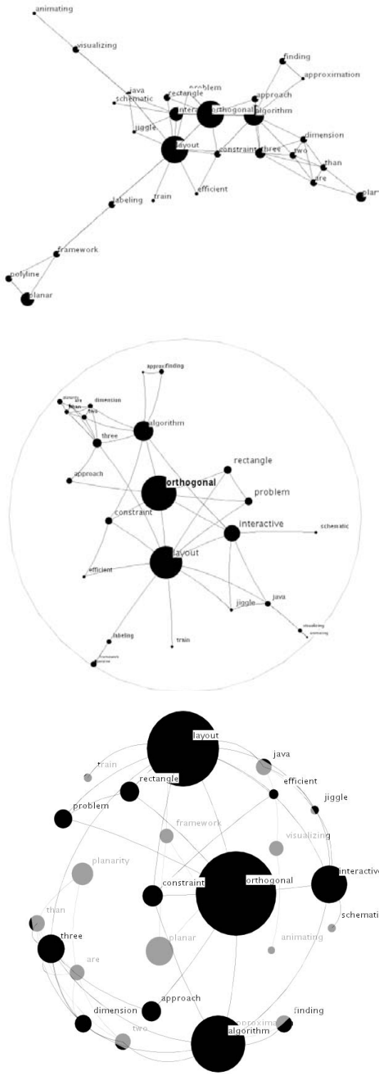
Figure 11: Layouts of the title-word graph, obtained in \mathbb{R}^2 , \mathbb{H}^2 and \mathbb{S}^2 . The graph has 27 nodes and 50 edges.
