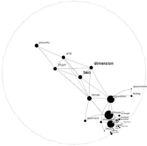
Figure 9: Layouts of the title-word graph with different centers of attention in hyperbolic space.
